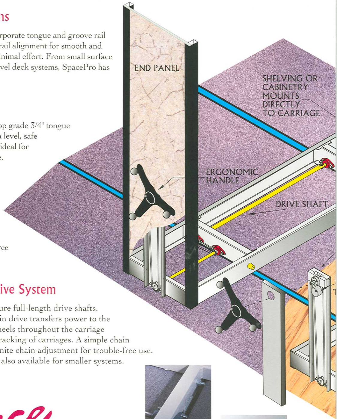
Unique one-piece welded wheel channels create the industry's strongest carriage framework
