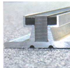
Neoprene track inserts eliminate debris collection allowing carriages to roll smoothly
